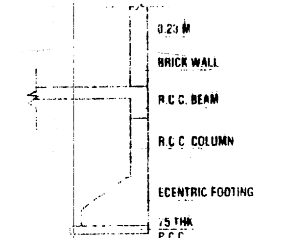
SECTION E.F. COMPOUND WALL DETAILS.
