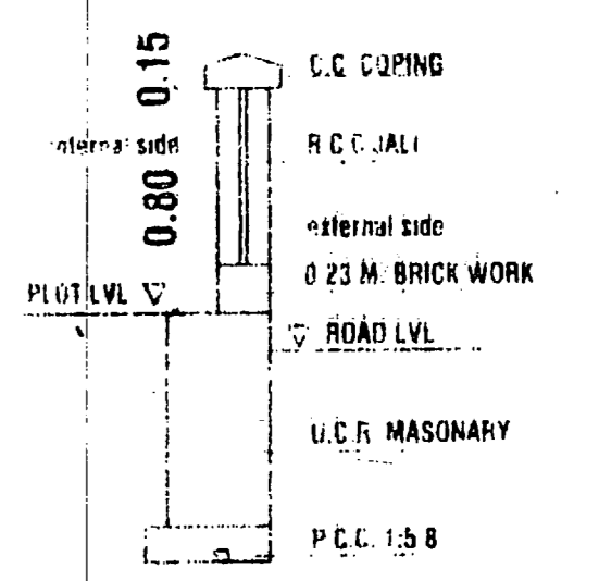
SECTION SECTION AT CORNER
