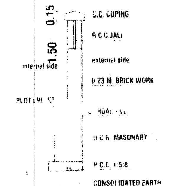
SECTION SECTION
