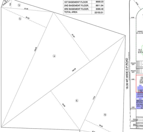
PLOT AREA DIAGRAM SCALE: 1:500
