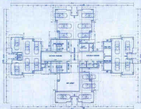
STILT FLOOR PLAN BLOCK - I (SCALE - 1:200)
