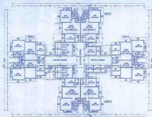
TYPICAL FLOOR PLAN (1st, 10th & 10th FLOOR) BLOCK - I (SCALE - 1:200)
