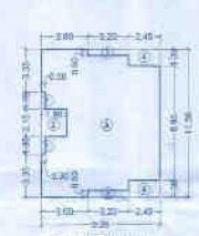
AREA LINE DIAGRAM TYPICAL 1st, 10th & 10th FLOOR BLOCK - B (SCALE - 1:200)
