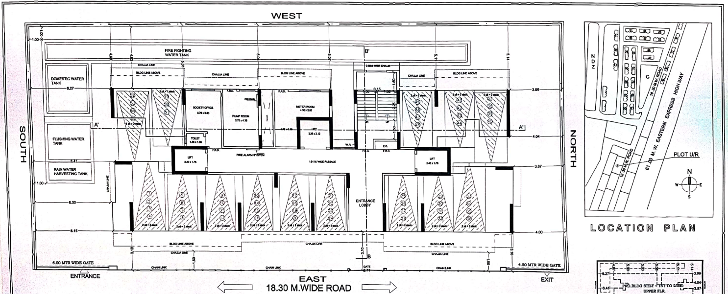
STILT FLOOR PLAN
