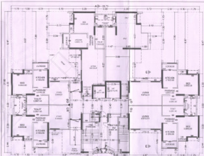
GROUND FLOOR PLAN CLUSTER 3.03 - A WING SCALE 1:100
