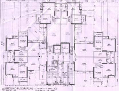
GROUND FLOOR PLAN CLUSTER 3.03 - C WING SCALE 1:100
