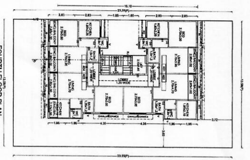
FOURTH FLOOR PLAN
