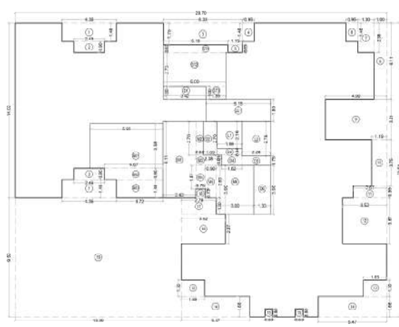
AREA DIAGRAM FOR GROUND FLOOR PLAN SCALE: 1/50
