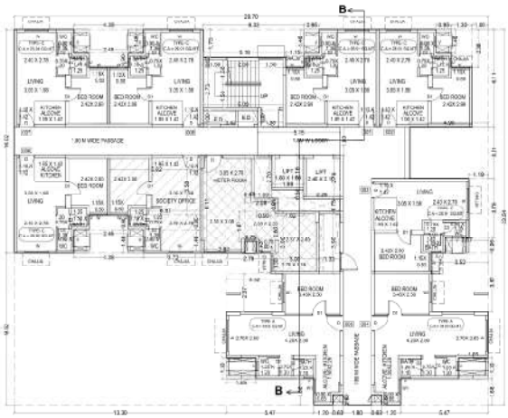
GROUND FLOOR PLAN SCALE: 1/50
