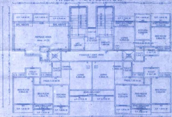
SEVENTH FLOOR PLAN
