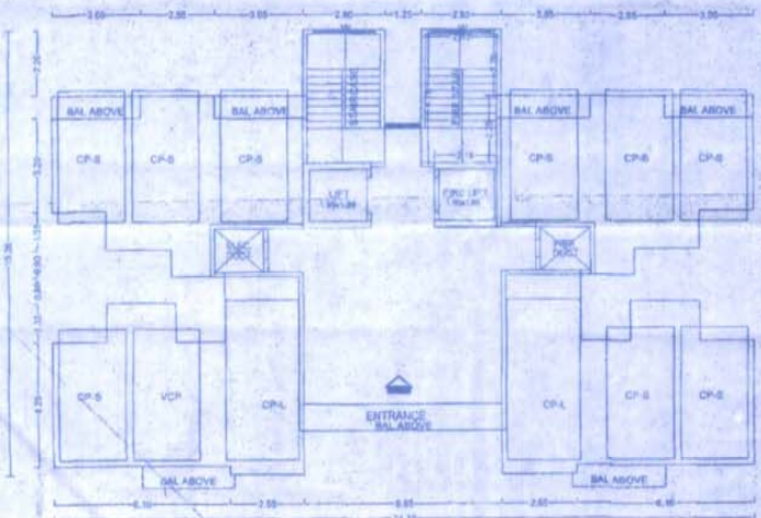
PODIUM FLOOR PLAN
