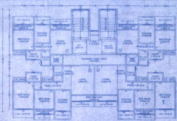
TYPICAL - 1, 6, 8 FLOOR PLAN
