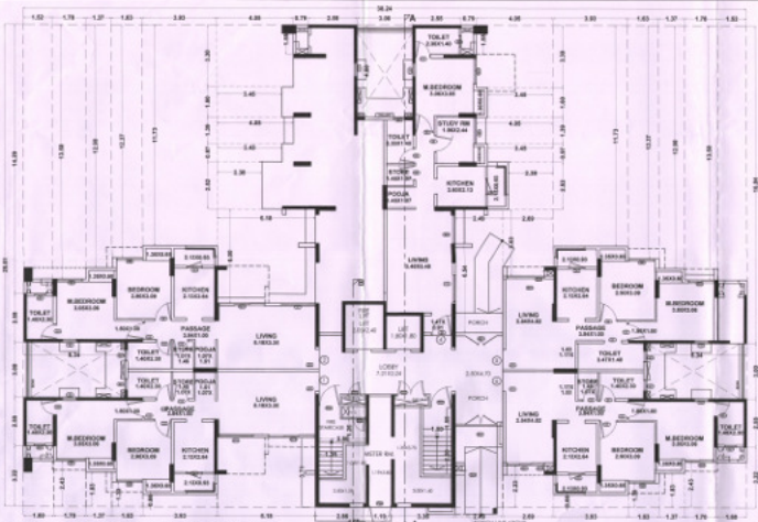
A GROUND FLOOR PLAN CLUSTER NO-1.05 (WING L, O) (WING O) SCALE: 1:100
