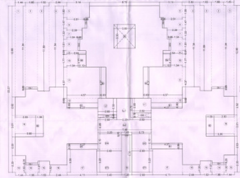
AREA LINE DIAGRAM OF 1ST TO 7TH, 9TH TO 12TH & 14TH TO 17TH FLOOR SCALE: 1:100
