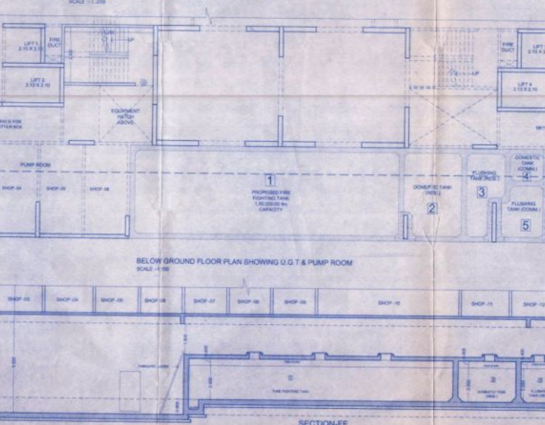
BELOW GROUND FLOOR PLAN SHOWING U.G.T & PUMP ROOM SCALE: 1:100
