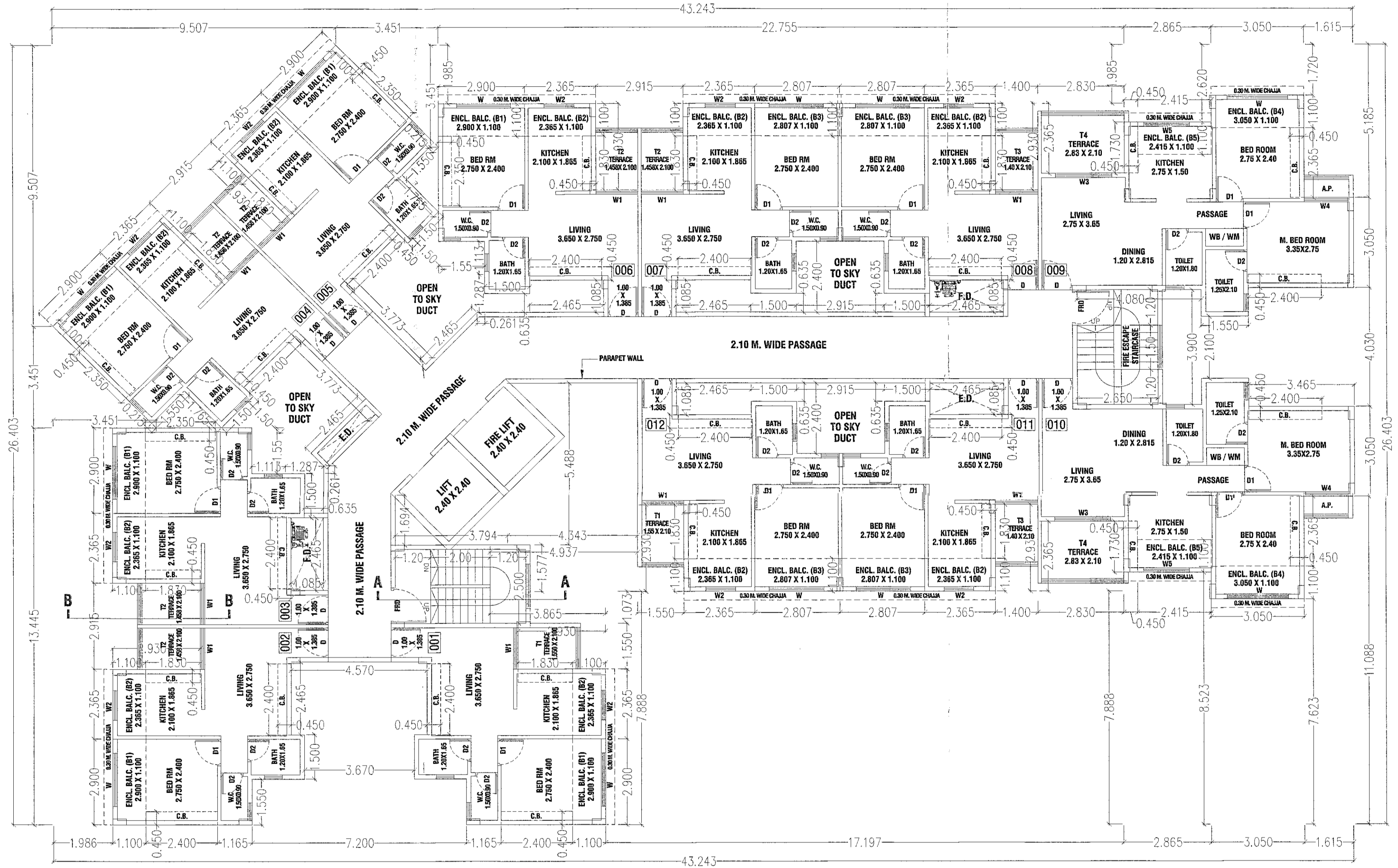
1ST, 3RD, 5TH FLOOR PLAN (BLDG. J) (SCALE = 1/100)
