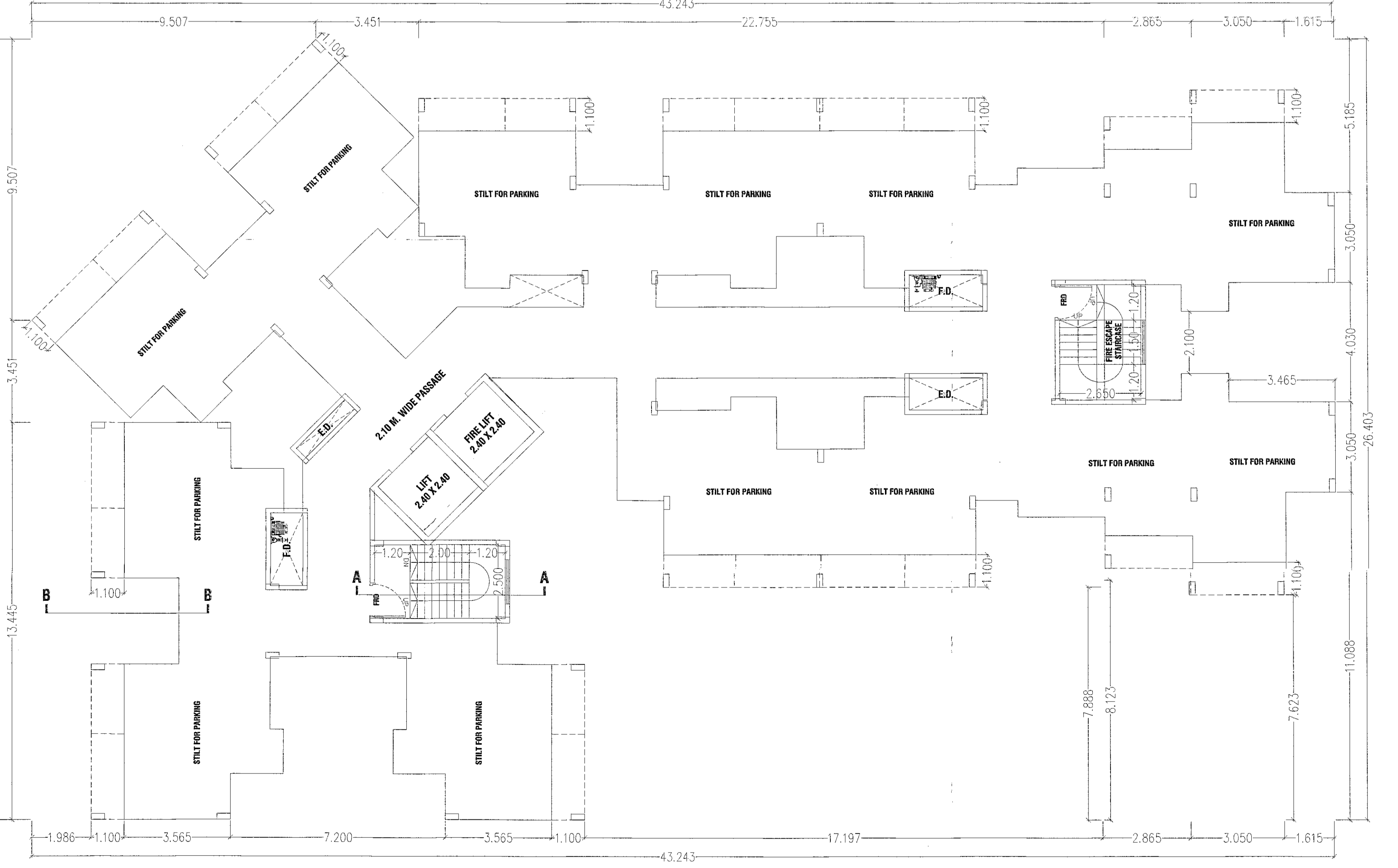
STILT FLOOR PLAN (BLDG. J) (SCALE = 1/100)
