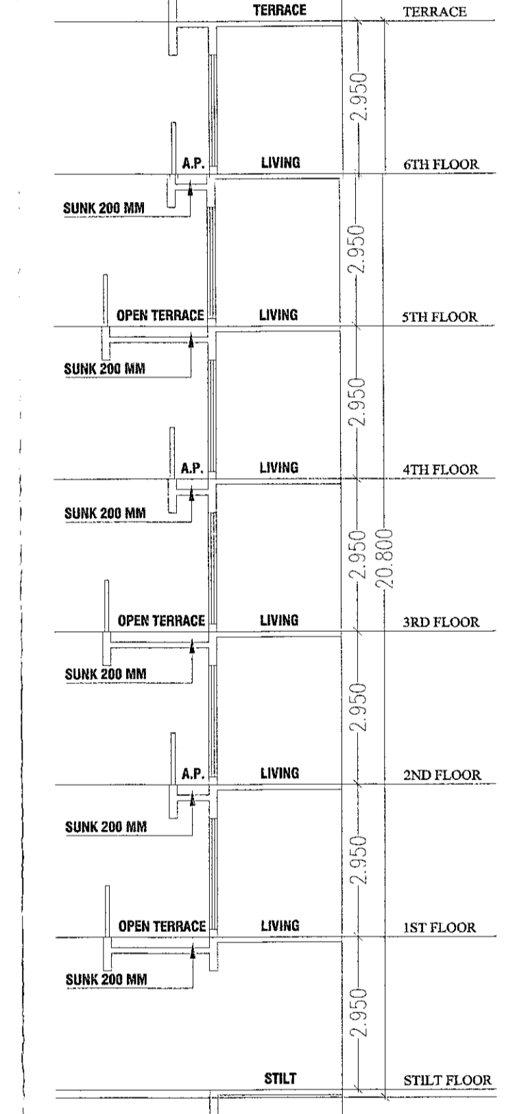
FRONT ELEVATION (BLDG. J) (SCALE = 1/100)
