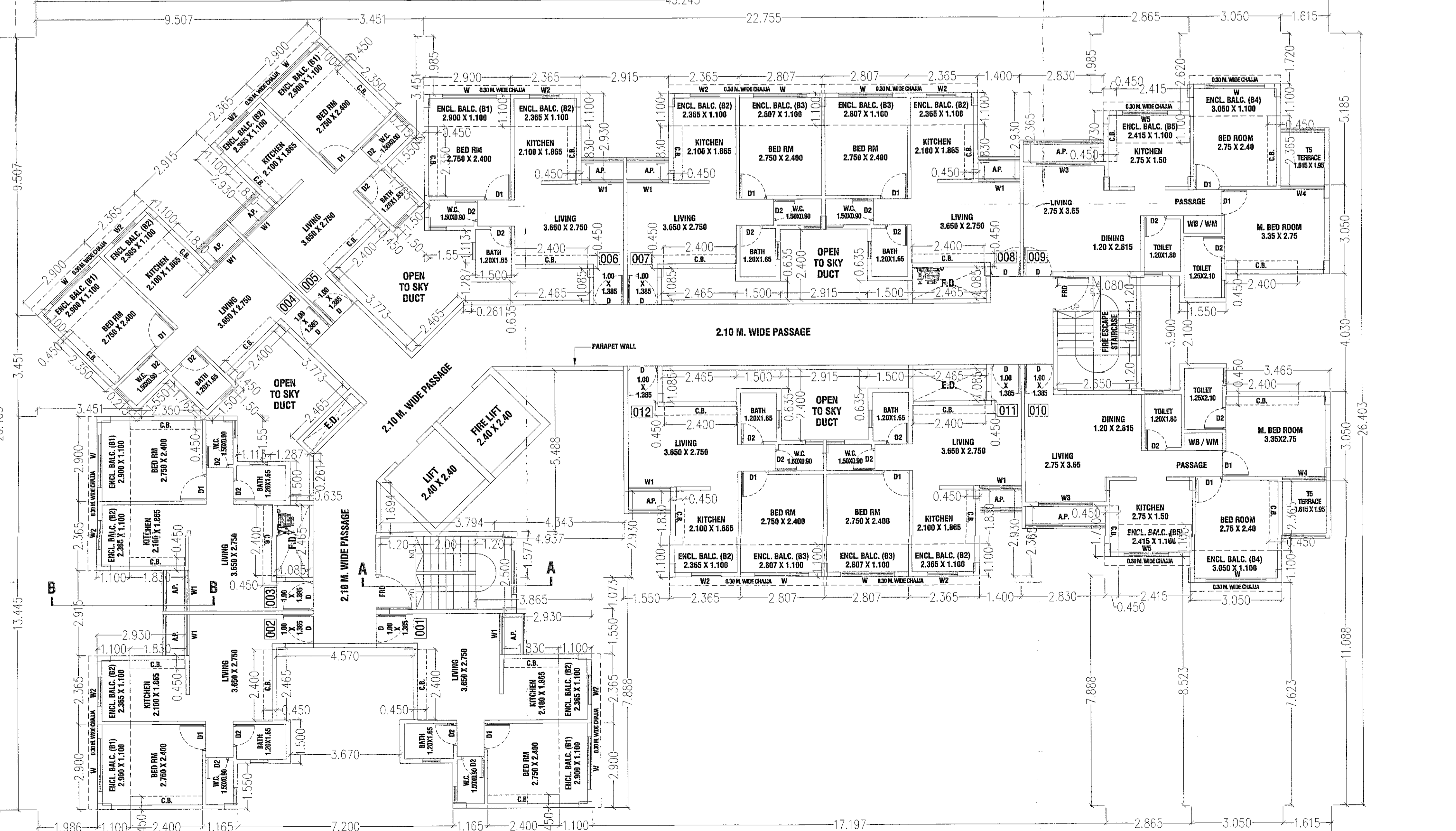
2ND, 4RD, 6TH FLOOR PLAN (BLDG. J) (SCALE = 1/100)
