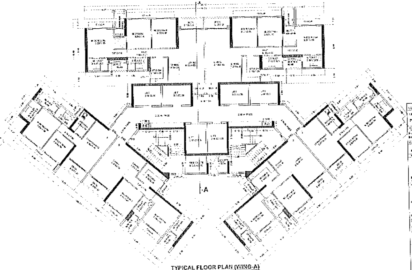
TYPICAL FLOOR PLAN (WING-A) 21st, 22nd & 23rd TO 25th SCALE - 1:125
