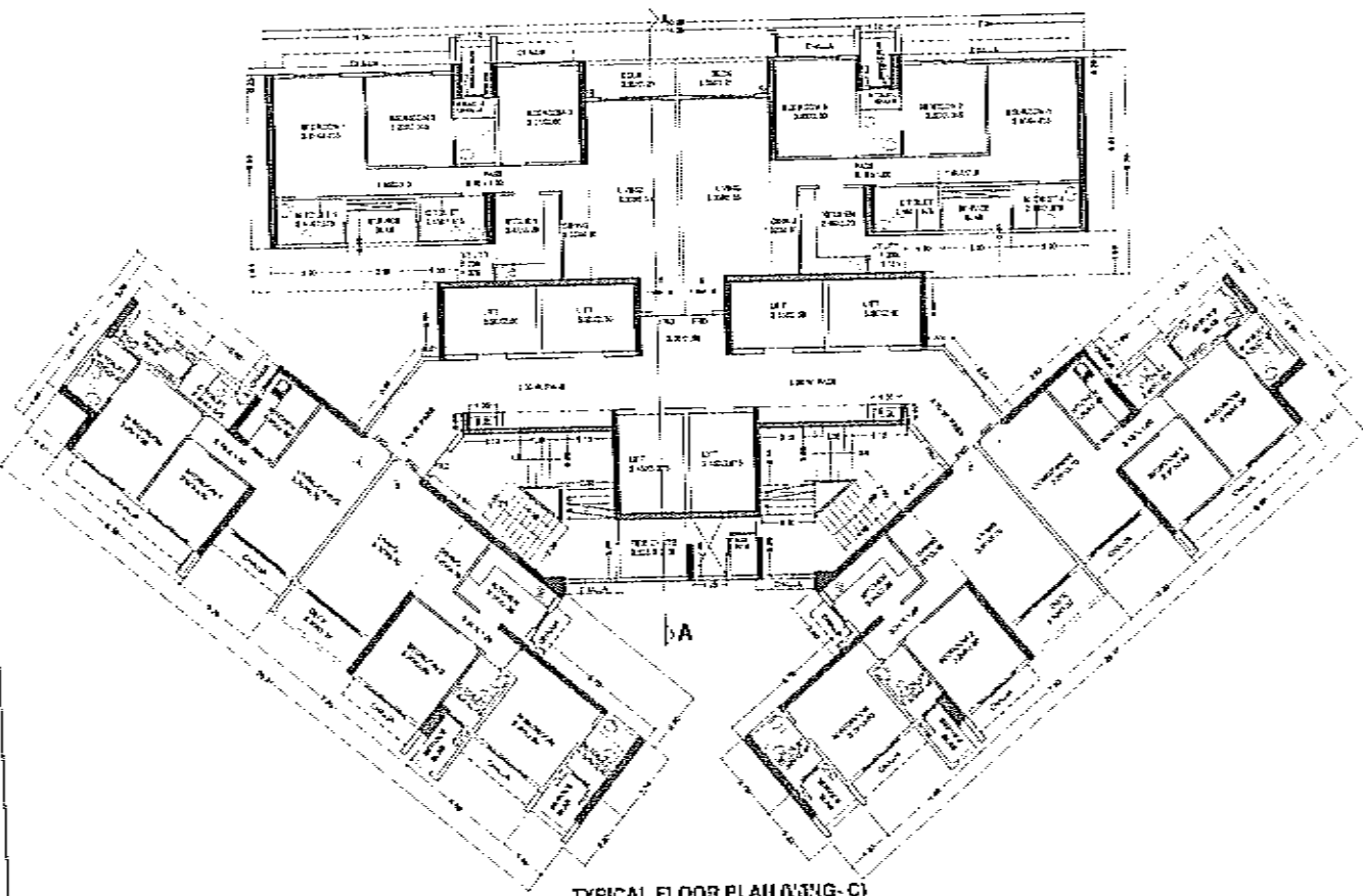
TYPICAL FLOOR PLAN (WING-C) 20 TO 21ST, 24TH TO 26TH, 28TH TO 31ST, 33RD & 34TH SCALE - 1:100
