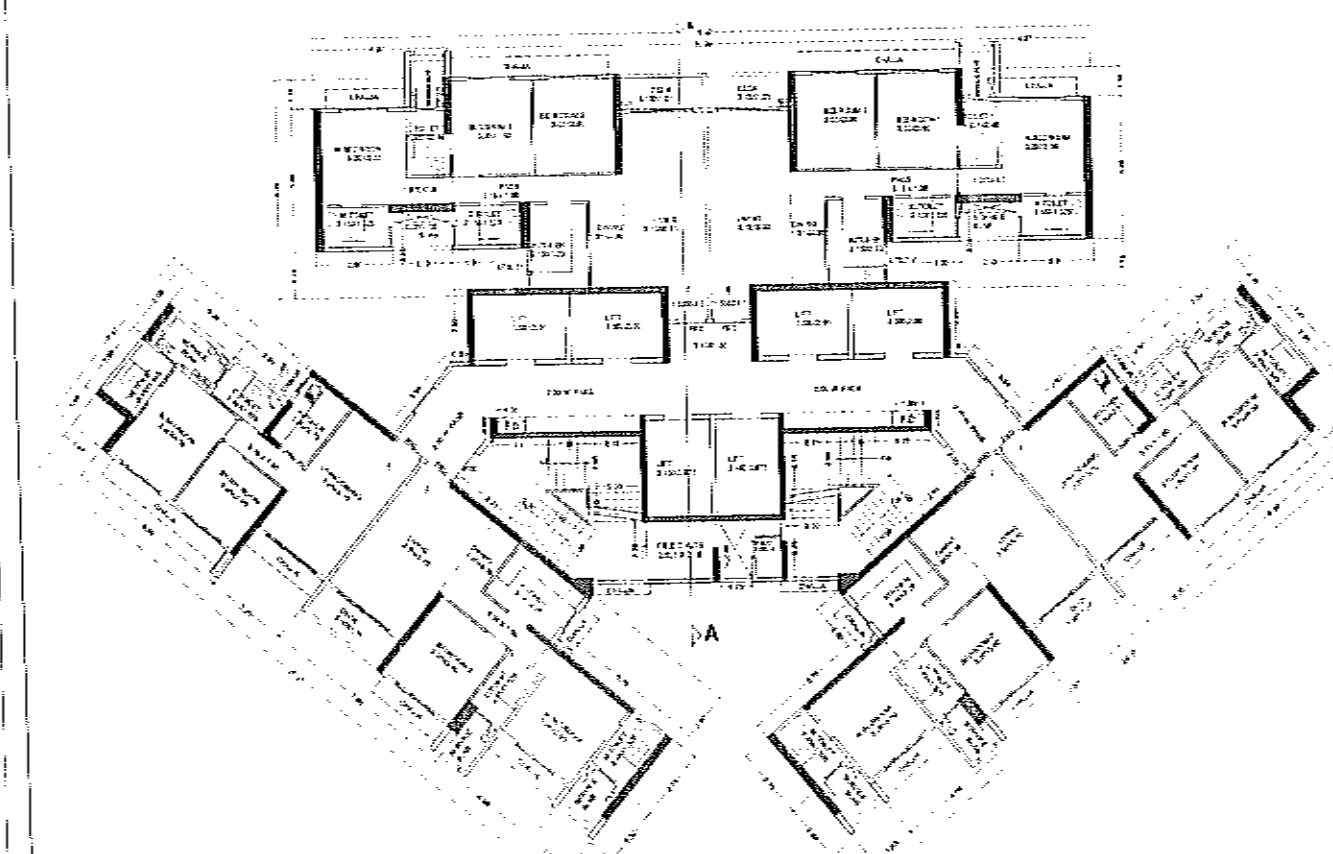
TYPICAL FLOOR PLAN (WING-A) 2nd TO 16th, 19th TO 21st, 18th TO 21st & 23rd TO 25th SCALE - 1:125
