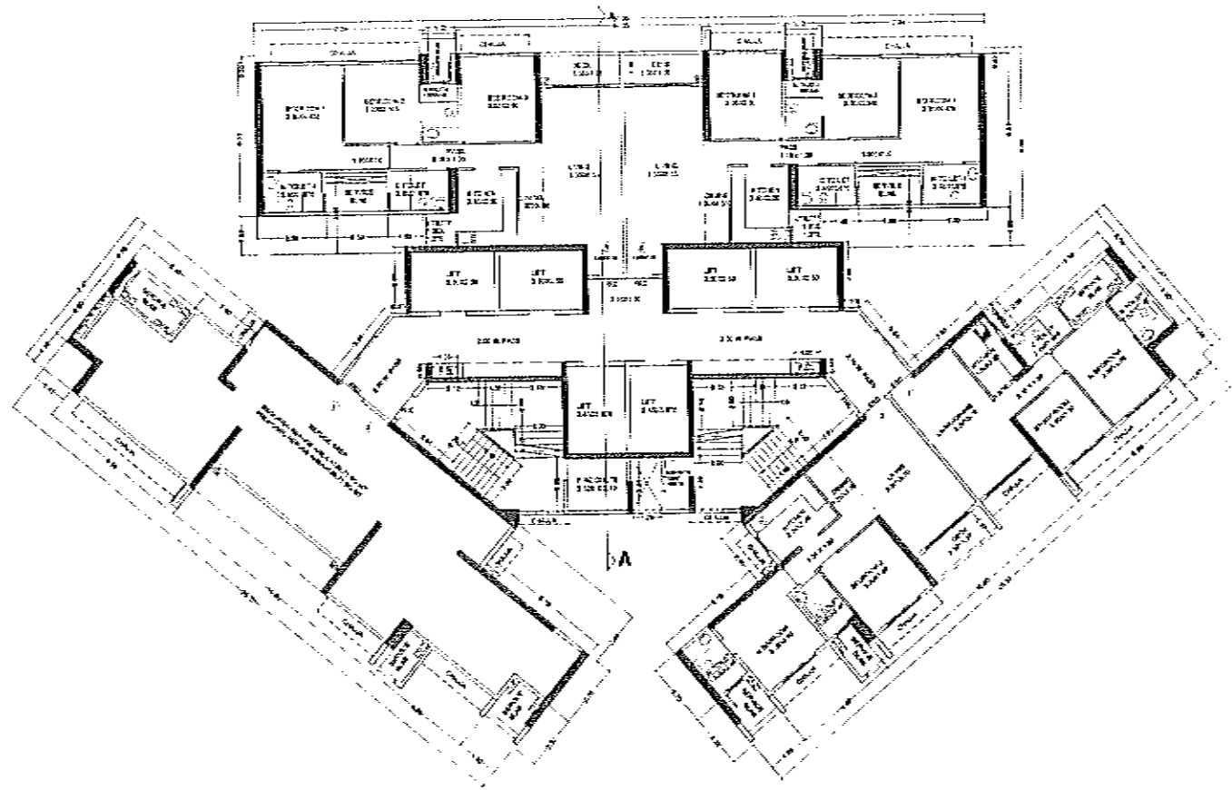
TYPICAL REFUGE FL. PLAN (WING-B) 1ST, 8TH, 15TH & 22ND FLOOR SCALE - 1/32"
