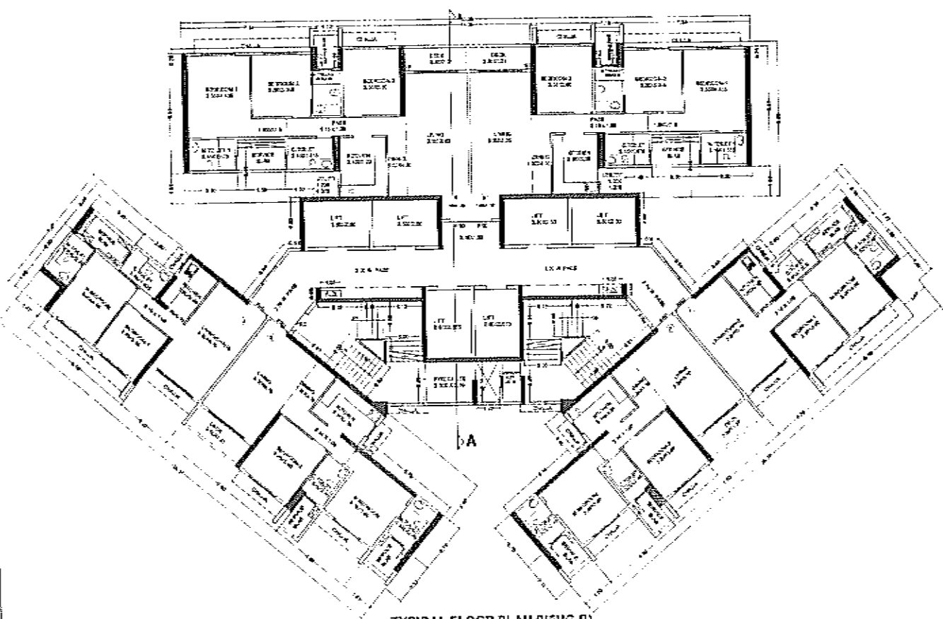
TYPICAL FLOOR PLAN (WING-B) 2ND TO 7TH, 9TH TO 14TH, 16TH TO 21ST & 23RD TO 28TH SCALE - 1/32"
