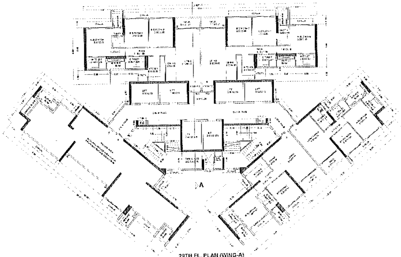
29TH FL. PLAN (WING-A) REFUGE FLOOR SCALE - 1:125
