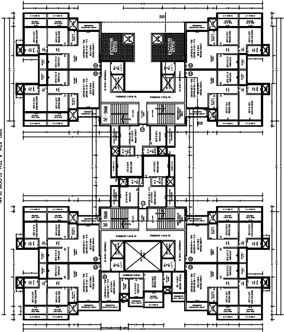
3RD, 5TH, & 7TH FLOOR PLAN (SCALE: 1:100)
