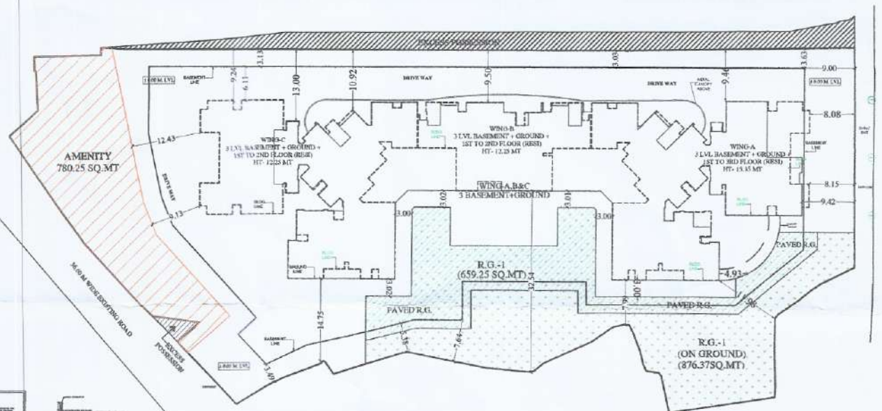
BLOCK PLAN SCALE 1:500
