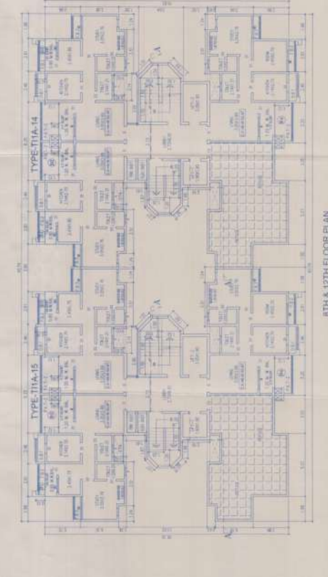
8TH & 12TH FLOOR PLAN
