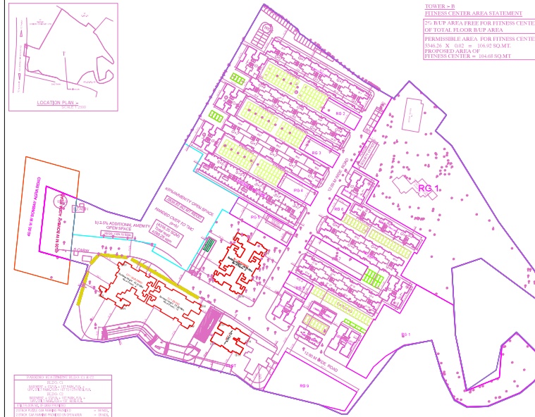
LAYOUT PLAN (Scale - 1:1000)
