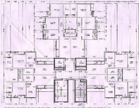
TYPICAL FLOOR PLAN 1ST TO 7TH, 9TH TO 12TH & 14TH TO 17TH FLOOR PLAN SCALE: 1:50
