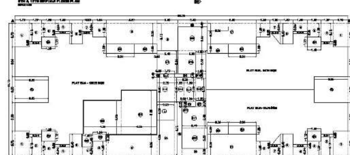
AREA LINE CHAIRMAN FOR 8TH & 13TH REFUGE FLOOR PLAN
