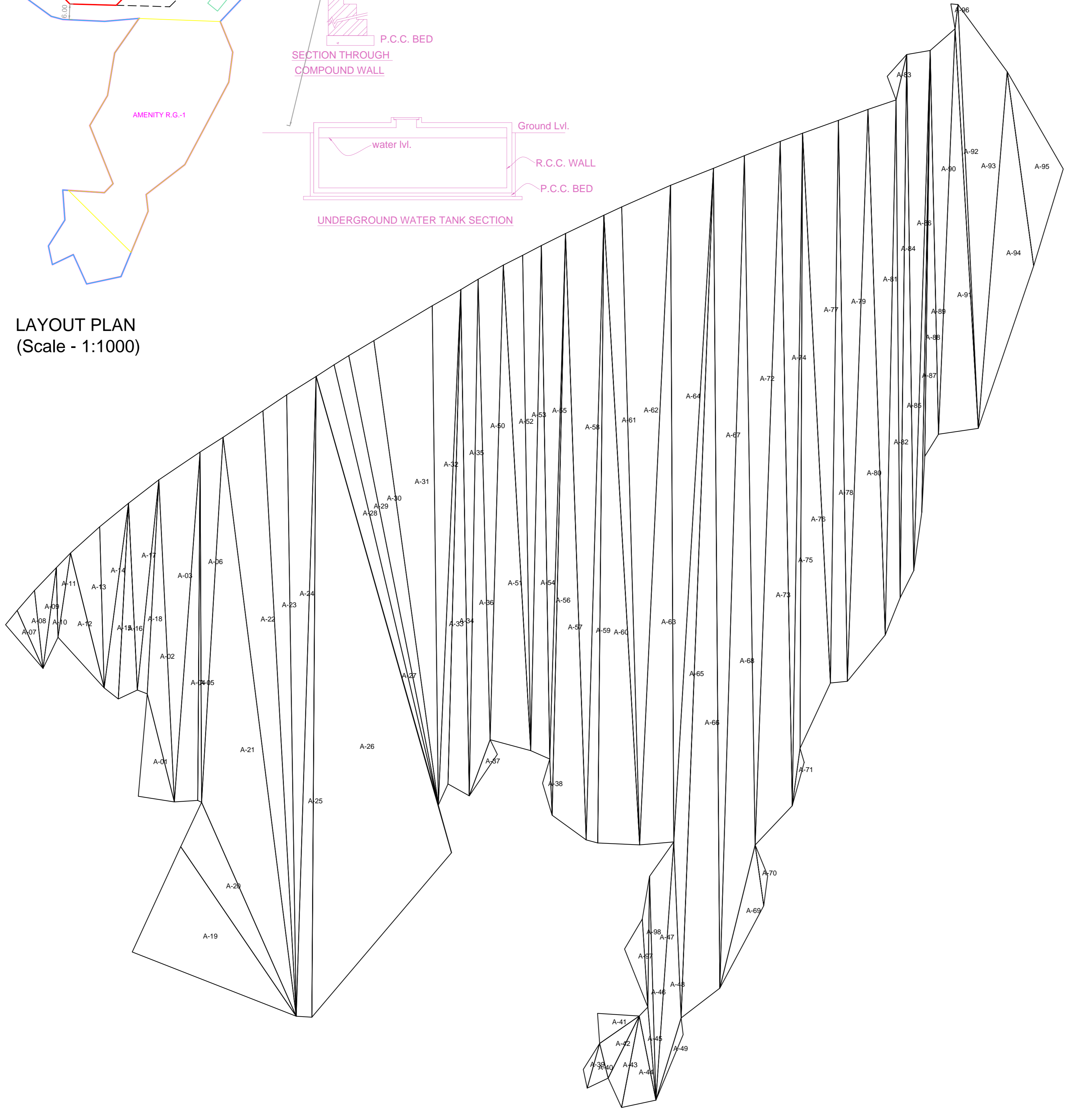
Triangulation (Scale - 1:1000)
