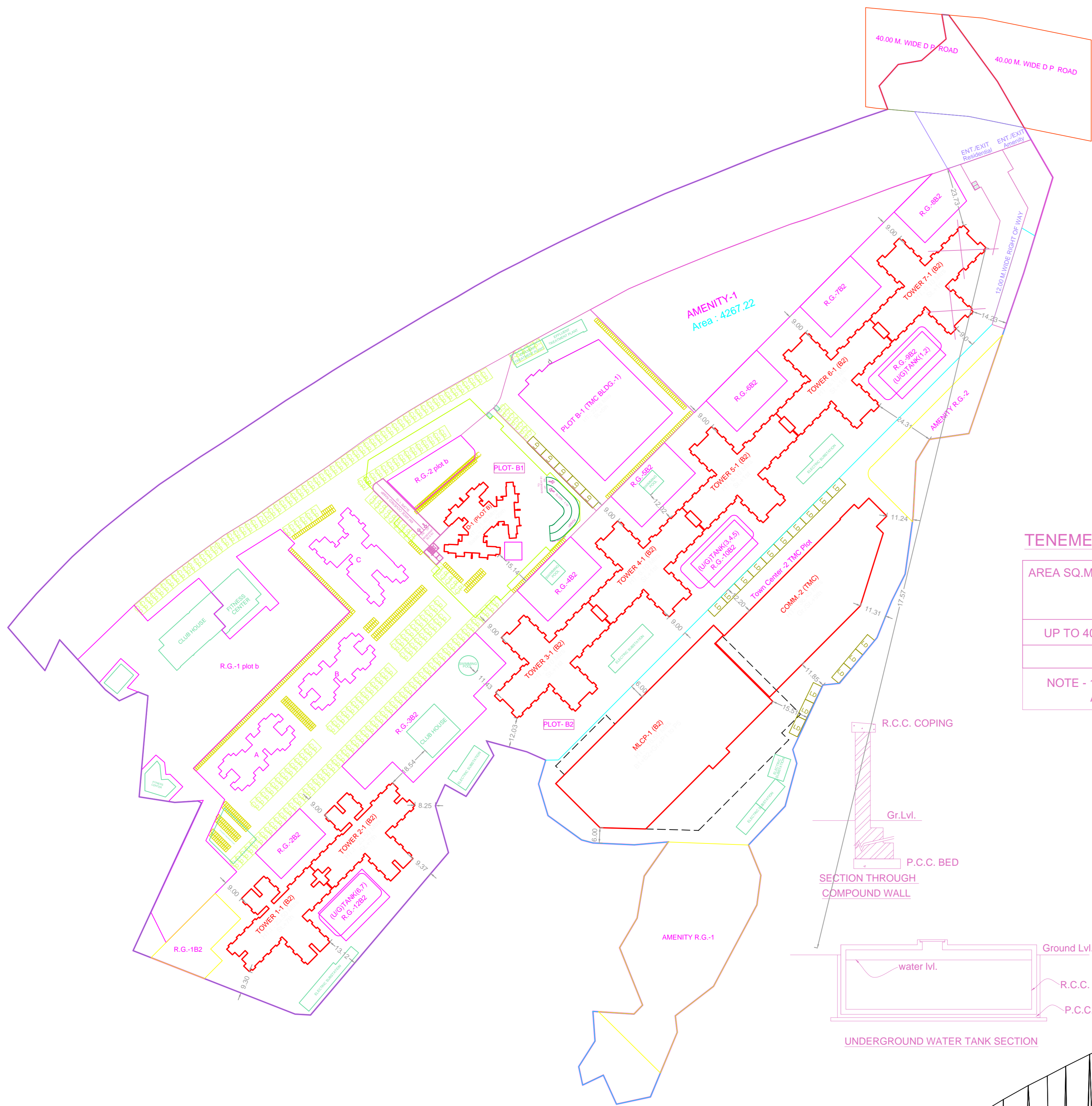
LAYOUT PLAN (Scale - 1:1000)
